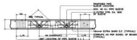
2 PIPE SLEEVE DETAIL @ BEAM
