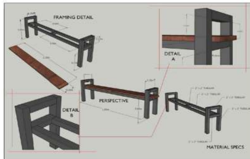
DINING BENCH DETAIL
