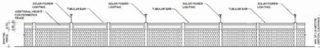
FENCE ELEVATION
