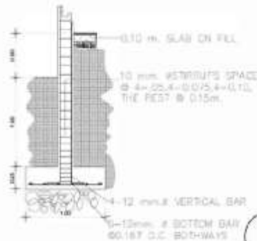
FENCE ELEVATION
