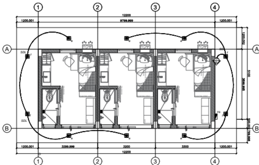
LIGHTING LAY OUT 2
